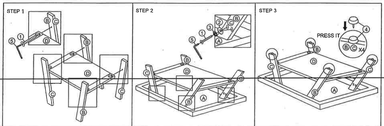
COMPLETED ASSEMBLE
